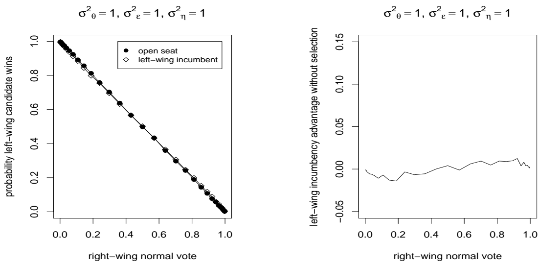
Figure 6: The left-hand panel shows the effect of partisan balance on the probability a left-wing incumbent wins, if there is no selection on quality, and the probability a left-wing candidate wins an open seat. The difference between these (shown in the right-hand panel) shows how partisan balance affects the left-wing incumbency advantage given the effects identified in Lemmata 4 and 5, but without electoral selection. Notice that the right-hand panel has the same vertical scale as the right-hand panel of Figure 3.
