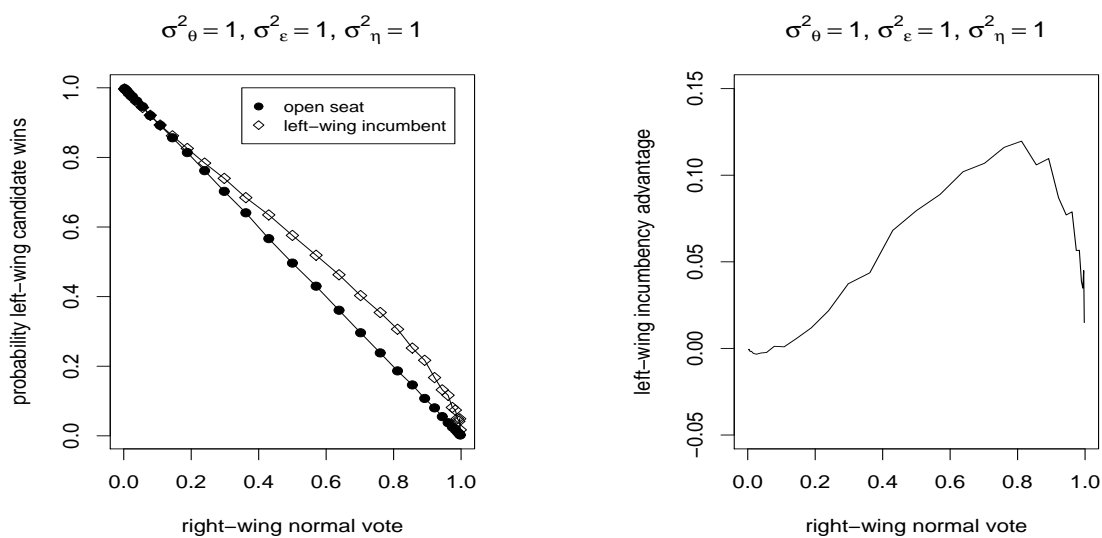
Figure 3: The left-hand panel shows how changes in partisan balance affect the simulated probability a left-wing candidate wins as an incumbent and in an open seat election. The right-hand panel shows how partisan balance affects the left-wing incumbency advantage—the difference between the two lines from the left-hand panel. The horizontal axis measures partisan balance as the probability that the right-wing candidate wins the open seat election. By a slight abuse of the standard terminology, we call this the “normal vote”—since, in our model, the probability of winning and the expected vote share have the same comparative statics, this should not cause any confusion.
