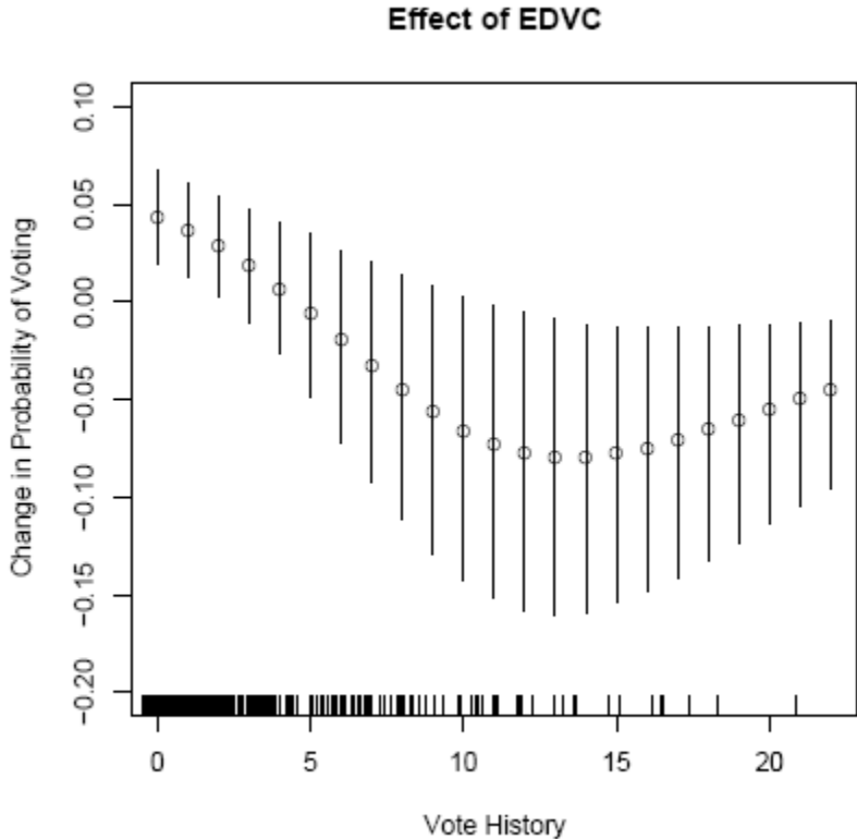
Figure 3: Effect of EDVC with 90% confidence bands
